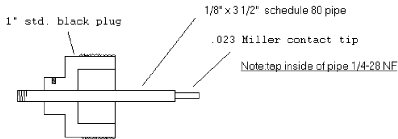
Cut away view of the 1" plug
